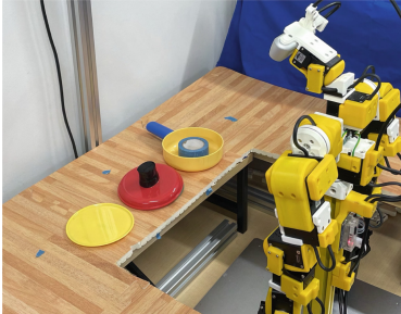
Fig. 3. Experimental environment (left) and the robot’s policies (right). The environment consists of a dual-arm robot (Rakuda-2), yellow and green plates, a yellow pot, a red lid, and a black ball and/or a white ball. Each policy is a sequence of actions that involves moving either the lid or one of the balls from one position to another.
