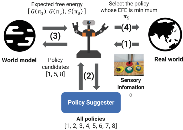
Fig. 1. Policy-selection steps in our proposed framework. (1) A robot acquires an initial observation from a camera mounted on it. (2) A policy suggester receives this observation as input and outputs policy candidates. (3) A world model is used to calculate EFE for each policy candidate. (4) The policy with the lowest EFE is selected, and the robot acts in the real world based on this policy.
