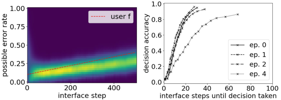
Fig. 8. Marginal belief distribution over channel statistics (left) and decision-making performance (right) of AINF AGENT with unknown control polarity and non-stationary channel statistics.
