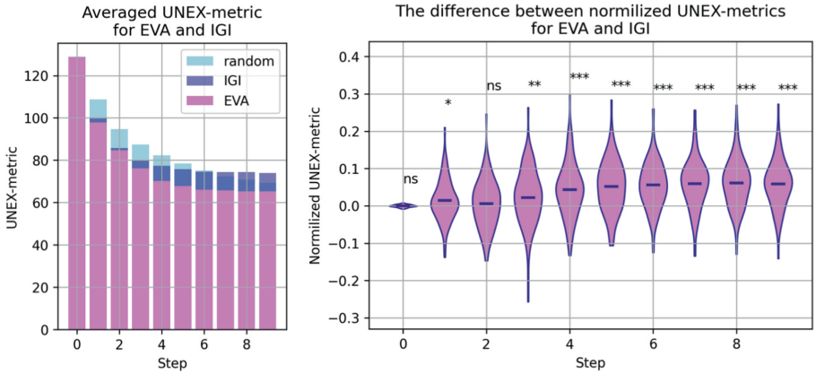
Fig. 7. The histogram (left) of the averaged across set of test digits UNEX-metric for three policies: random, IGI-based, EVA-based. The normalized UNEX-metrics distributions (right) with statistical significance indication
