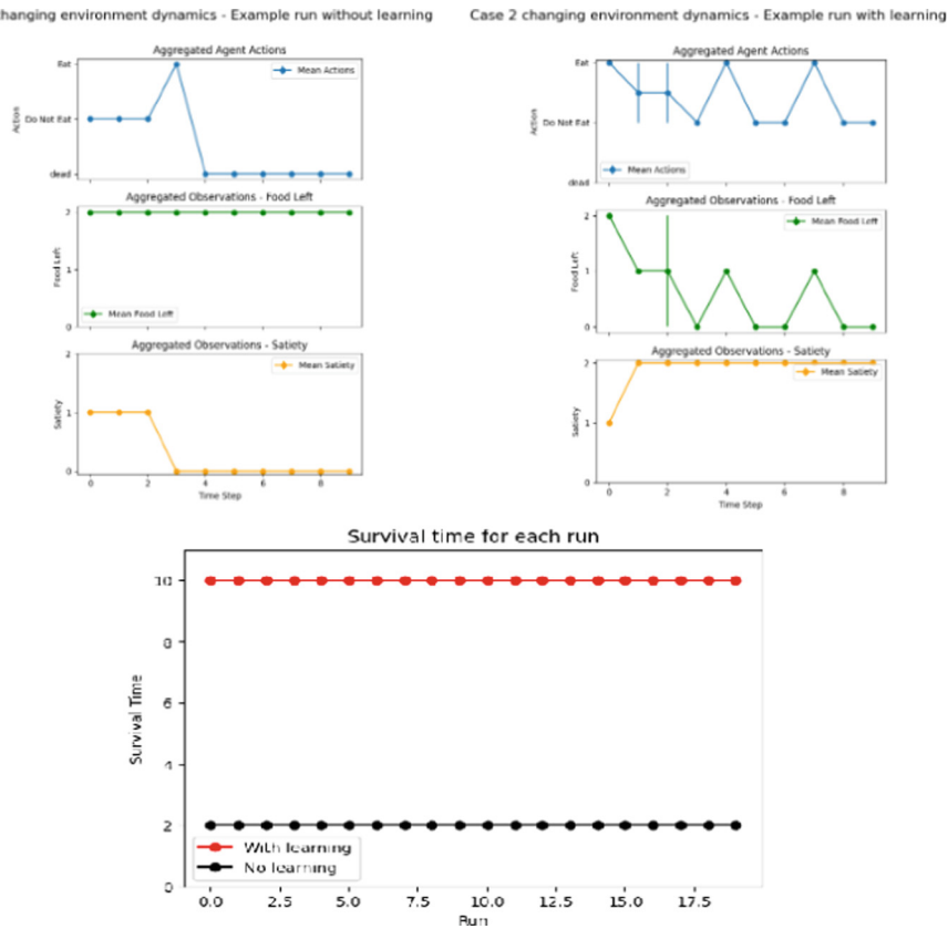
Fig. 8. Case 2 in a changing environment where food and satiety change at different time rates. The three top left plots show the results without learning off, and the three top right plots show the results with learning on. The bottom plot represents the comparison between the survival time over 10 time steps. Food increases at a slower rate (0.5 units per step) when not eating and decreases at a faster rate (1 unit per step) when eating. Satiety decreases faster when not eating (0.2 units per step) and increases at a different rate when eating (0.8 units per step).
