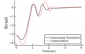
(c) Comparison of the evolution of the pole angle for the Unscented Transform and Linearization methods.
