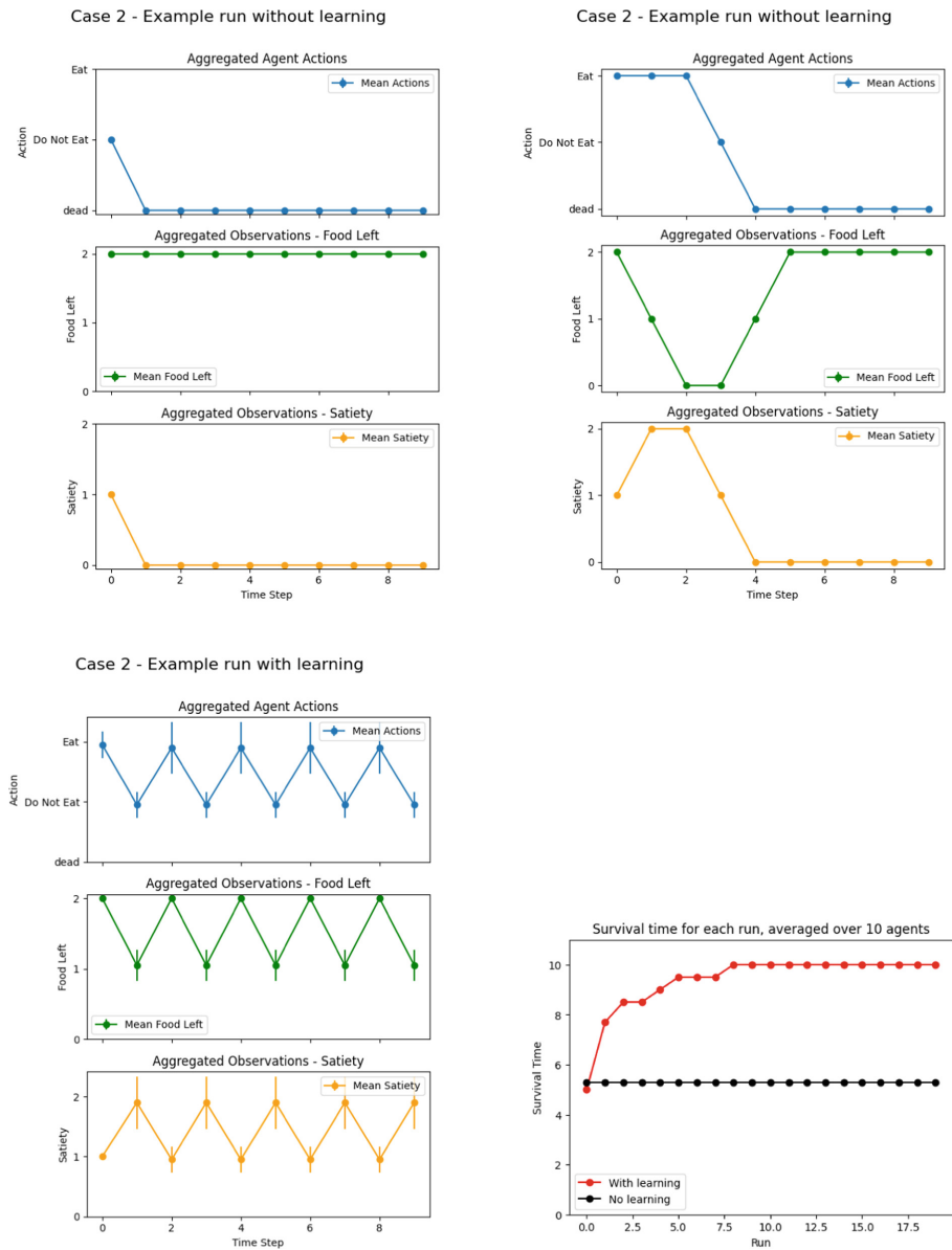
Fig. 4. Case 2 - Dynamic Environment. Without learning, the agent either does not eat (as shown in the three top plots on the left) or eats too much and therefore allows food in the environment to go to 0 (as shown in the three top plots on the right). As a result, the agent dies.
