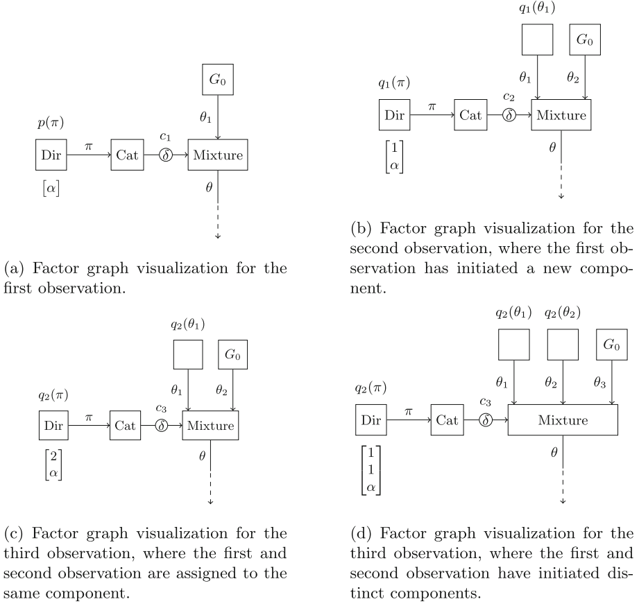
Fig. 2. Factor graphs of the initial time slices of the infinite mixture model of Sect. 3. The edge denoted by \theta here denotes the active or selected parameter settings. The edges connected to \theta have been dashed to highlight its extensibility towards arbitrary observation models. The parameter vector below the Dir-node denotes the simplified vector of concentration parameters.
