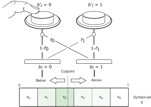
Fig. 2. The ordinal selection problem with noisy binary inputs (adapted from [20]). The user can emit one of two symbols, each with its own probability of flipping. Ordered target symbols are arranged on an interval. A cutpoint m_i is presented to elicit a binary “above/below” decision. A probability distribution over targets (green shading) is maintained during selection.
