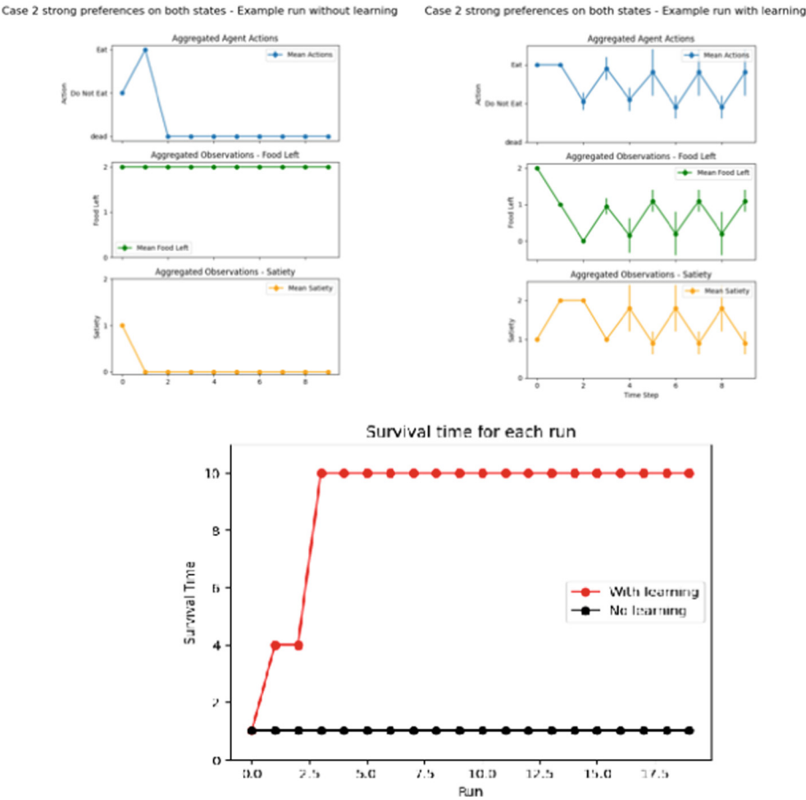
Fig. 7. Case 2 with strong prior preferences on both high satiety and high food left states. On the three top left plots, the agent has no learning, and on the top right, the agent has learning. On the bottom, we can see that survival time is vastly different with and without learning, as the preferences affect the behavior of the agent.
