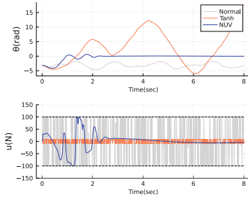
(a) Comparison of the evolution of pole angle \theta_t and inferred control u_t for three different control priors: normal, tanh constraint, and box-NUV.
