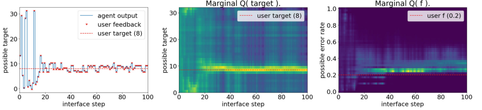
Fig. 3. Interaction between a simulated user with symmetric input error ( f_0 = f_1 = 0.2 ) and AINF AGENT with flat symmetric prior assuming no knowledge about input polarity Q_0(f_0) = \mathcal{U}(0, 1) , Q(f_1) = Q(f_0) . Left: Sequence of agent actions (blue), user input (red arrows), and user target (red dashed). Center: Marginal belief over user targets. Right: Marginal belief over channel statistics. Note that the belief over user target and channel statistics is in the continuous domain and is only discretized for visualisation purposes.
