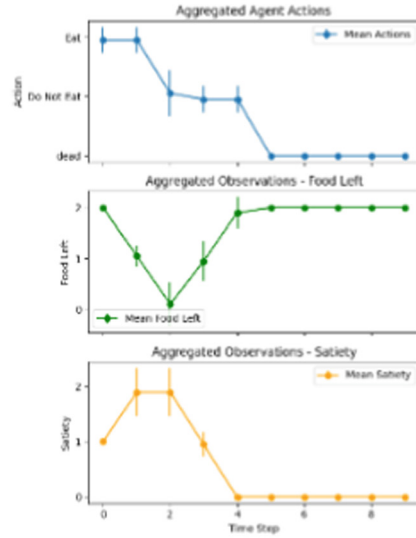
Case 2 policy length = 1 - Example run with learning
