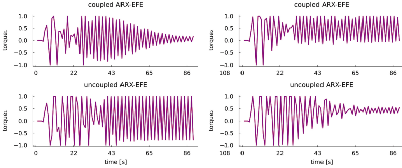
(b) Controls plotted over time. All agents exhibit a short inactivity phase in the beginning, before choosing non-zero controls. The control signals for both the coupled agent controlling mass m_1 and the uncoupled agent controlling mass m_2 have an initial period of large oscillations, which gradually diminish in amplitude, eventually converging to specific values (0.0 for the coupled agent, 0.4 for the uncoupled agent) with narrower oscillations.
