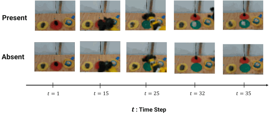
Fig. 4. Latent imagination results in an uncertain scenario. From the initial observation, it is unclear whether the environment contains the white ball under the red lid. The top row shows the result when the policy \pi_1 to open the lid was used for latent imagination, resulting in the appearance of the white ball on the green plate in the center. The bottom row shows the result with the same initial observation and policy, but without the appearance of the white ball on the green plate. (Color figure online)
