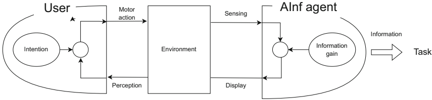
Fig. 1. An active inference agent whose goal is to extract intention from a user’s mind and pass it to some external task. The agent has sensing to determine environment states (some of which are influenced by the user) and display channels to influence the environment (some proportion of which are perceived by the user). The agent acts to reduce its uncertainty over user intention so that it can propagate this to the task.
