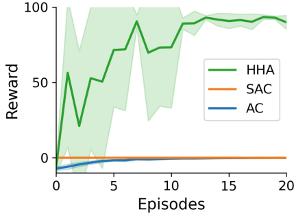
Fig. 6. HHA both finds the reward and capitilises on its experience significantly quicker than model-free RL baselines. Average reward ( \pm std) over 6 runs for Continuous Mountain Car (20 episodes, max episode length of 200 steps) for HHA (our model), Soft-Actor Critic (with 2 Q-functions), and Actor-Critic models. Note that after 20 episodes, SAC and AC are yet to find the reward and converge on a solution.
