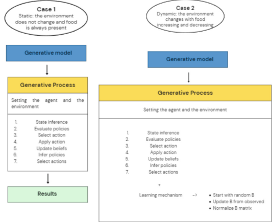
Fig. 2. Flowchart summarising case 1 and case 2 experimental setup.
