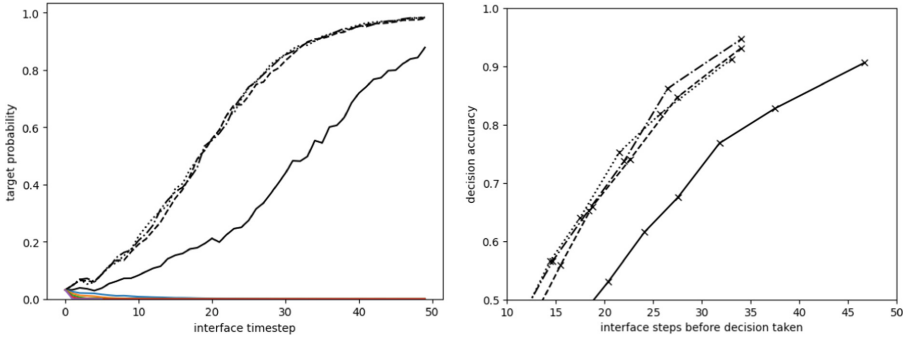
Fig. 7. Decision-making performance of AINF AGENT and Horstein’s algorithm with unknown control polarity . Median marginal belief probability of the true user target for f_0 = f_1 = 0.2 , varied assumed headroom f' - f for the Horstein algorithm, and sequential episodes for the AINF AGENT.
