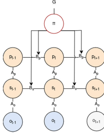
Fig. 2. factor graph POMDP of our generative model transitioning from past and present (up to time-step t ) to future (time-step t + 1 ). The pose p_t is inferred from the previous pose p_{t-1} and the action from policy \pi , while the state s_t determined by the corresponding observation o_t and influenced by the previous state s_{t-1} , pose p_t and action a_{t-1} . Past actions and observations are assumed observable, indicated by a blue colour. In the future, the actions are defined by a policy \pi influencing the new states and position in orange and new predictions in grey.
