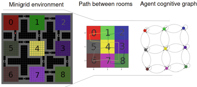
Fig. 1. From the mini-grid environment [3, 30] with different rooms annotated by colour to the path our agent took -from black to white- to form a successful exploration correctly linking all the rooms up to the agent’s internal topological graph with the state associated to each room.
