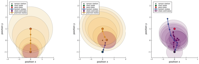
Fig. 1. (Left) Planned trajectory at k = 1 , from start to goal directly over the sensor station. (Middle) Planned trajectory at k = 5 showing a mismatch between true and estimated state resulting in a strong adjustment to the planned trajectory. (Right) Executed trajectory over a trial of 10 steps demonstrates the agent losing track of the robot when it approaches the sensor station.
