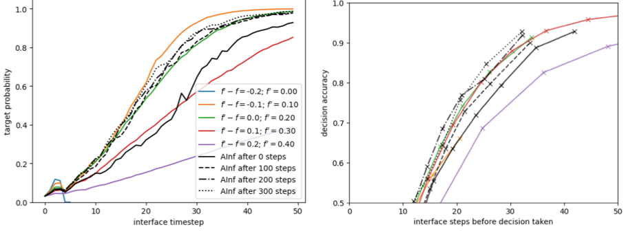
Fig. 6. Decision-making performance of AINF AGENT and Horstein’s algorithm with known control polarity . Median marginal belief probability of the true user target for f_0 = f_1 = 0.2 , varied assumed headroom f' - f for the Horstein algorithm, and sequential episodes for the AINF AGENT.
