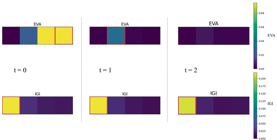
Fig. 5. Illustration of IG estimated by two methods: EVA (upper) and IGI (lower). The red frame indicates the action chosen by the agent based on the maximal IG value. (Color figure online)
