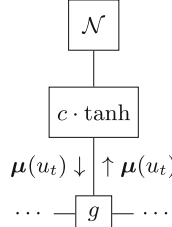
(b) FFG for control constraints via the hyperbolic tangent function.
