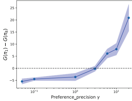
Fig. 6. Difference in EFE between two policies when the preference precision is varied. The horizontal axis represents the preference precision, and the vertical axis shows the EFE difference between policy \pi_1 (opening the pot lid) and \pi_8 (moving the ball from the left to the right pot), denoted as G(\pi_1) - G(\pi_8) . Solid points indicate the mean across five trials, with shaded areas representing the standard deviation.
