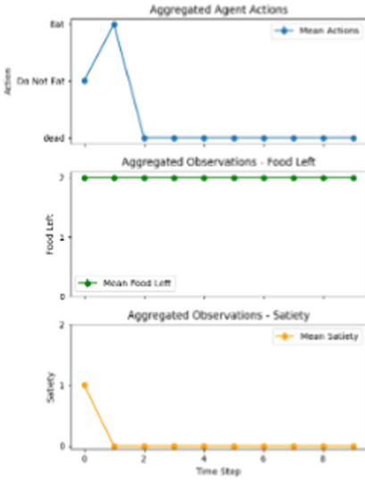
Case 2 policy length = 1 - Example run without learning
