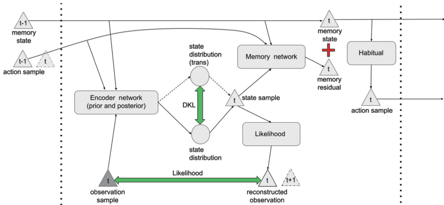
Fig. 3. The schematic representation of the DAI model used. Triangles represent generated samples, circle - Gaussian distributions, green arrows - FE loss (EFE is not represented), rectangles - neural networks. Note in the MNIST environment the auxiliary reconstructor network was used also which is not drawn for clarity. (Color figure online)
