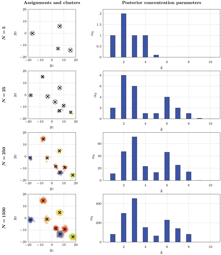
Fig. 3. Visualization of the results obtained by performing online inference in the infinite mixture model defined in Sect. 3 using the message passing implementation as described in Sect. 4. Each row represents the number of observations N . The left column shows the observations colored by their inferred cluster label and the inferred component means, denoted by square crosses. The right column denotes the concentration parameters of the approximate posterior distribution q_N(\pi) .
