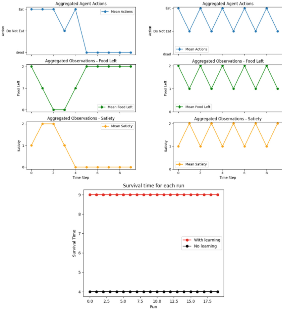
Fig. 6. Example run from Case 2 without learning enabled on the left and with learning enabled on the right, but starting with an extreme B matrix setting (probabilities set to 1 or 0, on the left three plots and middle three plots, and high but non-extreme values on the right). The agent dies quickly, just as the randomly set values of the B matrix in plot 6, and is able to learn on the right.
