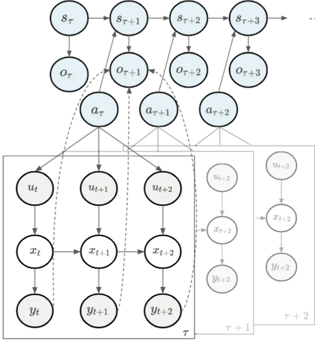
Fig. 1. Previous discrete-continuous active inference models have focused on the physical implementation of categorical decisions in continuous space. Here, outcomes from the high-level active inference planner select from a set of discrete models of continuous dynamics, specified by a prior over their hidden causes. This mixed generative model effectively generates discrete sequences of short continuous trajectories defined in terms of their generalised coordinates of motion. The discrete planner is formulated as a standard POMDP generative model (see Sect. 3.3) with discrete states s_\tau and observations o_\tau . The first action a_\tau of the selected policy (see Sect. 3.2) is then passed down to the continuous active inference controller via the expected observation q(o_{\tau+1}|a_\tau) . This distribution weights a set of fixed point means \{\eta_m\}_{m=0}^{M-1} which map the m discrete latent states into continuous state space. The resulting weighted average, \eta_\tau = \sum_m \eta_m \cdot q(o_{\tau+1,m}|a) , serves as the mean of a prior over hidden causes, p(\nu) = \mathcal{N}(\eta_\tau, \pi_\tau^{-1}) , which drives the dynamics of the low-level continuous latent states \tilde{x}_t = \{x_t, x'_t, x''_t\} and observations \tilde{y}_t = \{y_t, x'_t, x''_t\} represented in generalised coordinates. Inherently, there is a separation of timescales in this open-loop control setup: the discrete controller sends an action down to the continuous controller which is then executed in a ballistic manner over several timesteps. After this low-level inner-loop completes, a process of Bayesian model selection is used to infer the current discrete state description of the low-level system given the trajectory of continuous observations \tilde{y}_t . This is then given as an observation for the discrete planner at the top. For a full treatment of this model, see [13].
