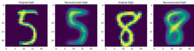
Fig. 4. Two examples of the original digits from the MNIST dataset reconstructed by DAI model after 30 steps with a random policy
