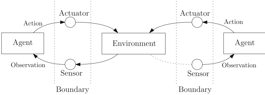
Fig. 1. General communication protocol in an Active Inference environment containing two agents. The terms “Actuator” and “Sensor” are used from the agents’ points of view. We see that both agents have a boundary with actuators and sensors with which they interact with the environment.
