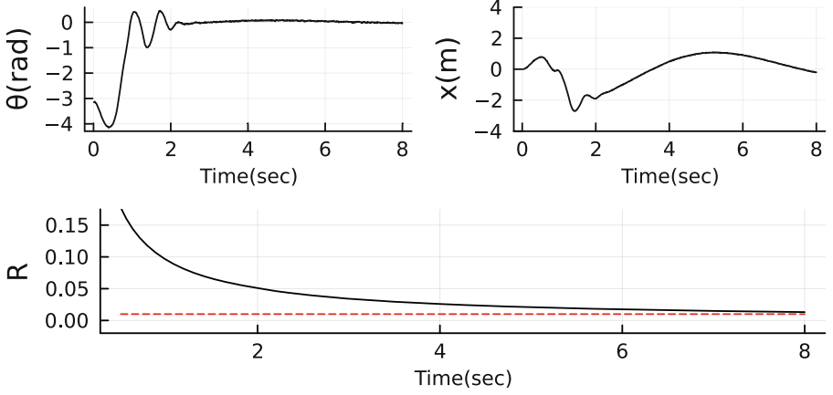
Fig. 2. Evolution of the pole angle (top-left), cart position (top-right), and inferred noise variance (bottom) over time. The dashed red line is the true added noise ( R^* = 0.01 ). (Color figure online)
