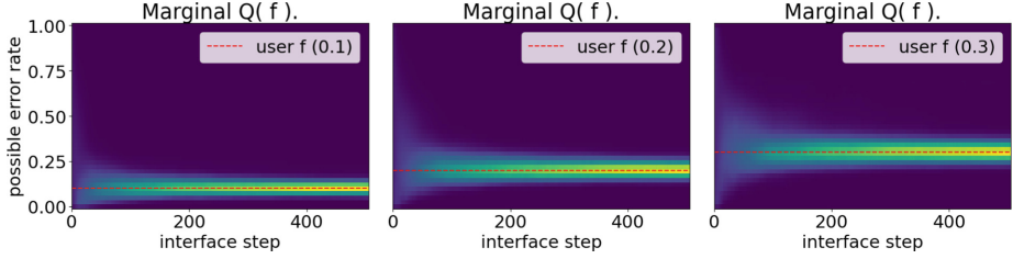
Fig. 4. Marginal probability of the true channel statistics under the belief distribution. Mean marginal belief distribution across all 32 user targets and 10 repetitions each over five successive interaction episodes of 100 steps. The belief converges around the true channel statistics within 100 to 300 steps, with higher error rates taking longer to infer.
