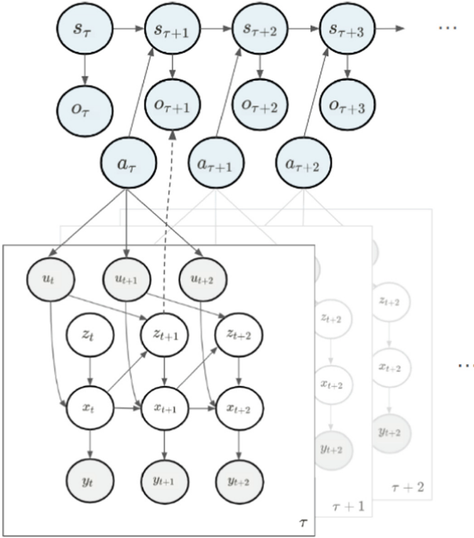
Fig. 3. Our Hybrid Hierarchical Agent learns emergent coarse-grained descriptions of the continuous state-space for planning and control. Like previous work on mixed generative models in active inference shown in Fig. 1, we have a discrete active inference planner sitting above a low-level continuous active inference controller. The discrete planner is constructed as a standard POMDP generative model (see Sec. 3.3) with discrete states s_\tau and observations o_\tau . However, our model departs from [13] in the generation of coarse-grained variables which instead emerge from the underlying rSLDS generative model. Here, the states S of the planner are essentially a re-description of the discrete states Z found by the rSLDS. The transition model probabilities are then constrained to reflect the adjacency structure of the polyhedral partitions of the state-space found by the softmax regression component of rSLDS. The chosen action a_\tau from the high-level planner selects from a discrete set of continuous active inference controllers based on both the linear dynamics of the current discrete state z_\tau and a control prior for the desired next discrete state. Using the rSLDS generative model, this prior is a flexibly specified continuous point in the state-space that is in the discrete region the agent wishes to move into (see Eq. 10). Unlike the models in [13], the action a_\tau is temporally abstracted with no pre-defined timescale at the lower level. Instead, the discrete planner is only re-triggered when the system enters a new discrete state (i.e. z_t \neq z_{t-1} ). At which point, the planner observes the new discrete state z_\tau of the system and constructs a plan accordingly.
