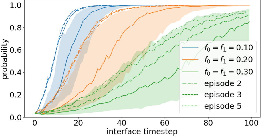
Fig. 5. Marginal probability of the true user target under the belief distribution. Shown are the median and inter-quartile range across all 32 user targets and 10 repetitions in the first 100 interaction steps, and the median across successive interaction episodes. Target inference speed converges after 1–3 episodes demonstrating the saturating effect of inferring the channel statistics.
