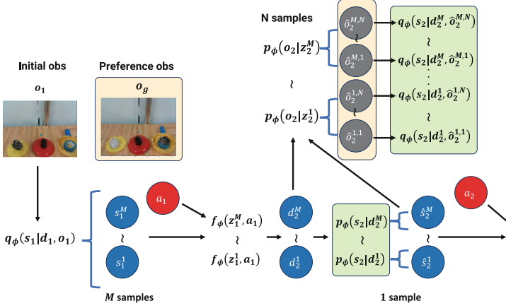
Fig. 2. Calculation of the approximate EFE. We first compute q_\phi(s_1 | d_1, o_1) from o_1 and sample \{s_1^i\}_{i=1}^M . From these and a_1 , \{d_2^i\}_{i=1}^M are computed. We then compute \{p_\phi(s_2 | d_2^i)\}_{i=1}^M and sample \{\hat{s}_2^i\}_{i=1}^M . Using \{z_2^i\}_{i=1}^M , we compute \{p_\phi(o_2 | z_2^i)\}_{i=1}^M and sample \{\hat{o}_2^{i,j}\}_{j=1}^N . Finally, we compute \{q_\phi(s_2 | d_2^i, \hat{o}_2^{i,j})\}_{j=1}^N .
