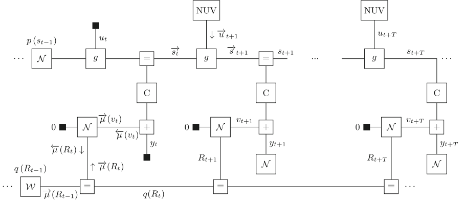
Fig. 1. A Forney-style factor graph representation of the probabilistic control model in (11). This snapshot illustrates the model at the time step t , with T future time horizon.
