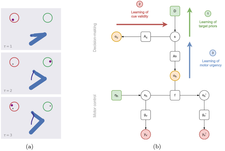
Fig. 1. Embodied decision setup and active inference model. (a) Experimental setup, during three consecutive discrete time steps \tau . The agent controls a 3-DoF arm, which starts at a home position (blue dot) at an equal distance from the two targets (red and green circles). The current cue is displayed with a big purple dot, while the old cues are shown with smaller grey dots. For each trial, the agent has to reach the target it believes will contain more cues. (b) Factor graph of a hybrid active inference model for embodied decisions. Variables and factors are indicated by circles and squares, respectively. We highlighted three pathways related to the learning of the correct target (green arrow), cue validity (red arrow), and response strategy (blue arrow). (Color figure online)
