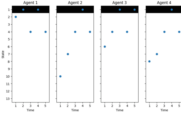
Fig. 4. Simulation of self-doubt for 4 agents. Again, each panel displays the evolution of the posterior belief as a function of time, where darker colors indicates a higher degree of belief. Blue dots indicate the agent location. All agents are initialized with a strong prior belief that the object will be at location 1, as indicated by the dark shaded area. This reflects a potential situation where all agents have been acting in the environment for a long time, accruing faulty evidence. In this case the communication mechanism prohibits the agents from discovering that the object is not there, even after observing its absence multiple times.
