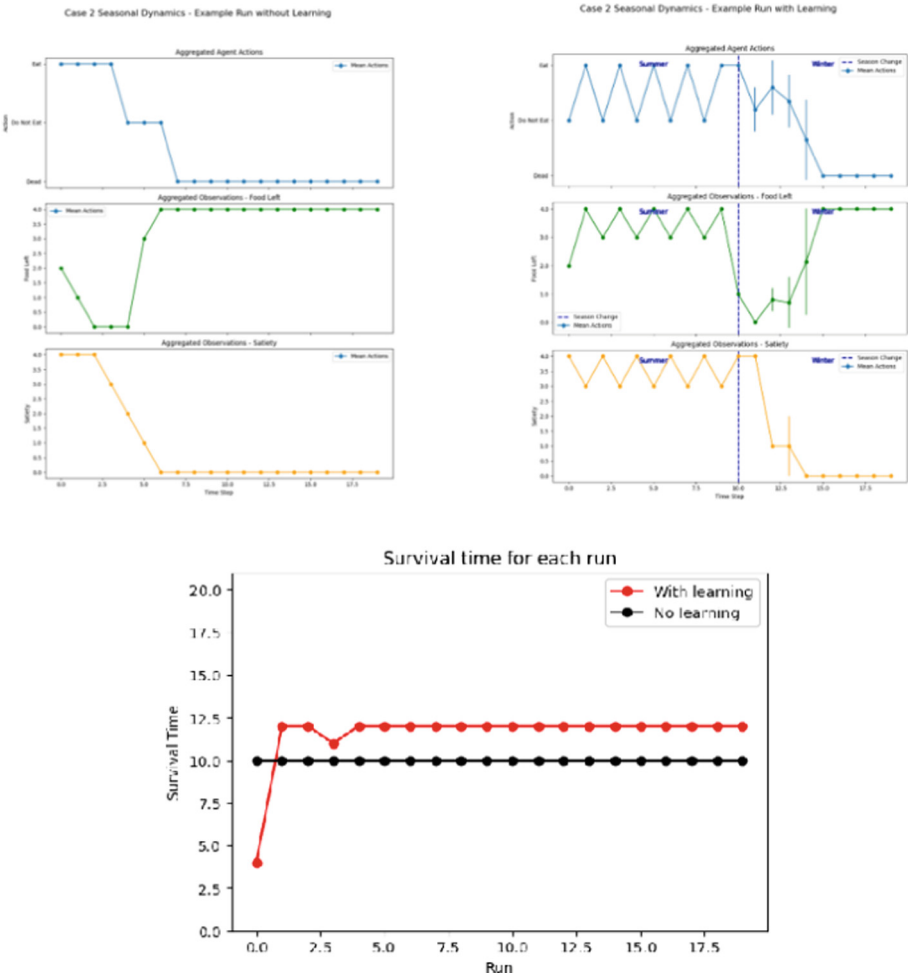
Fig. 9. Case 2 in a changing environment with seasonal simulation. The environment is built to simulate switching seasons summer/winter. With learning off the agent is not able to survive throughout the first season (top left plot and bottom plot). With learning on, it survives but then quickly dies throughout winter (top right plot).
