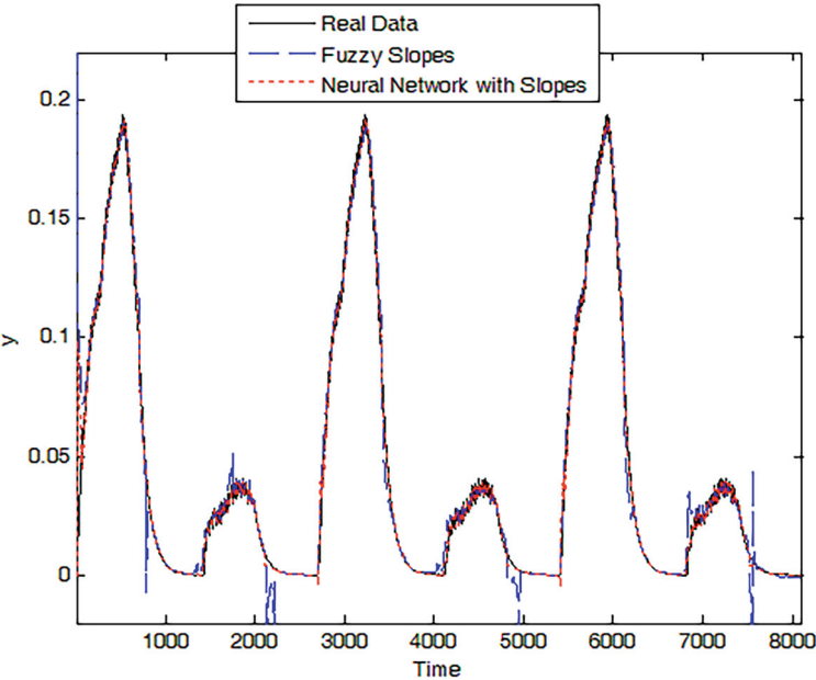
Fig. 4.10 Modeling for the training of experiment 2
