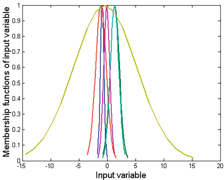
Fig. 7.10 Membership functions for Example 7.2
