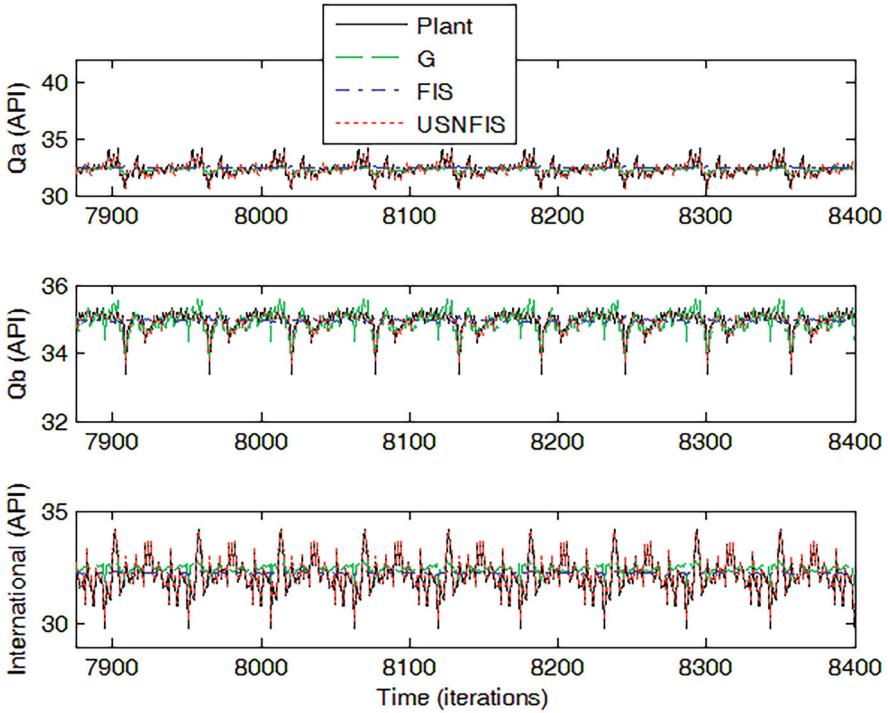
Fig. 6.4 Testing results for the oil blending process
