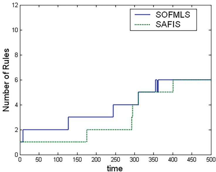
Fig. 7.9 Growth of rules for 500 iterations for Example 7.2
