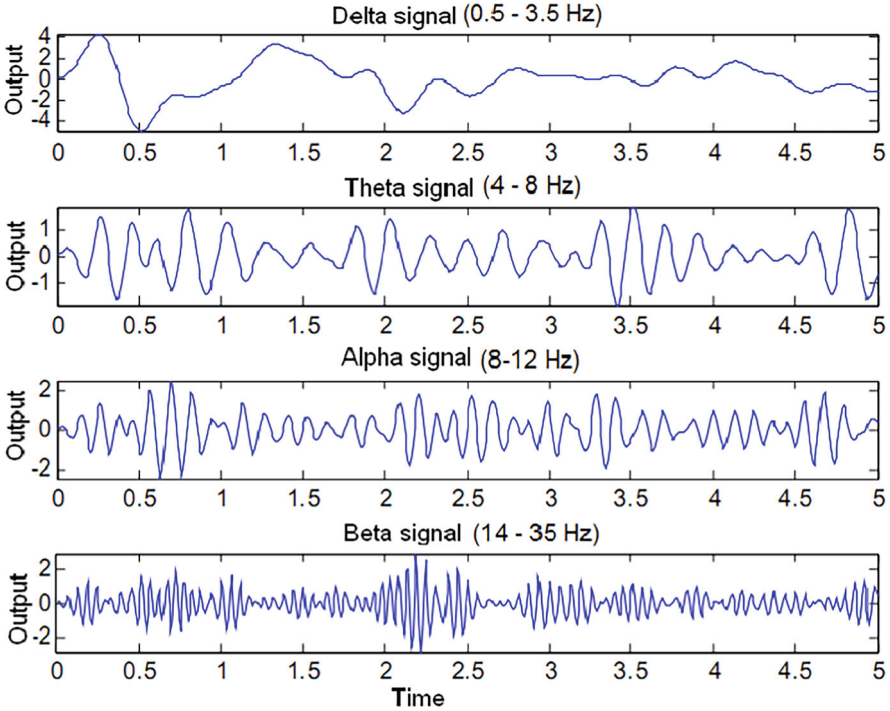
Fig. 10.1 EEG signals
