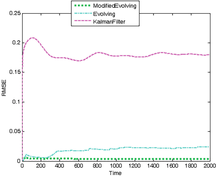
Fig. 8.6 The RMSE
