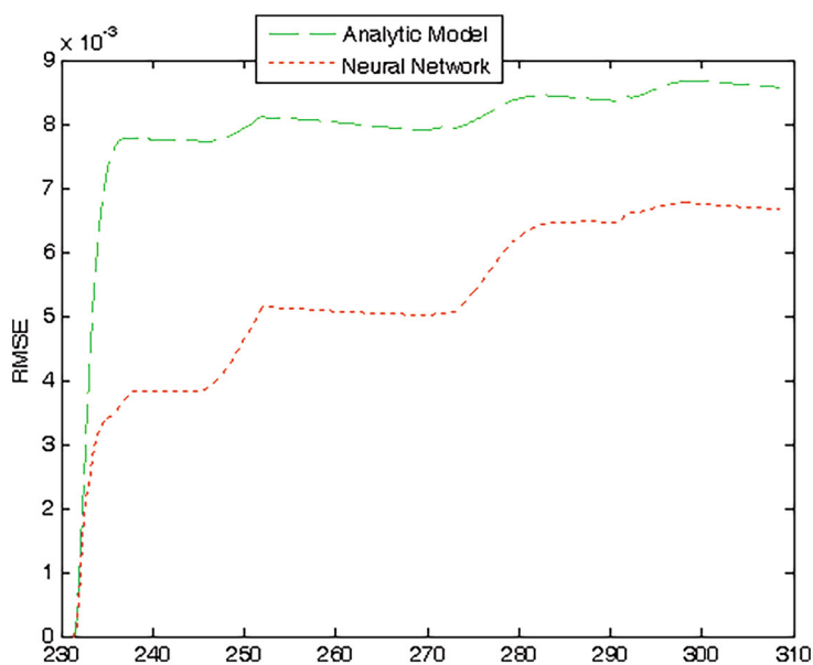
Fig. 3.7 RMSE for the testing of Example 1
